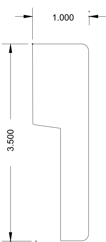
MB 6053 (3-1/2 x 1)
