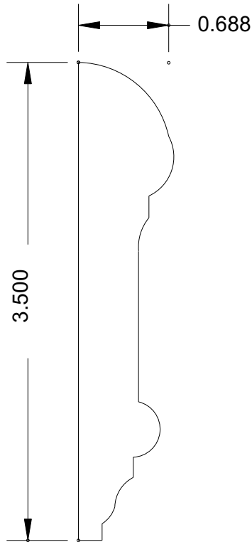
MB 281 (3-1/2 x 11/16)
