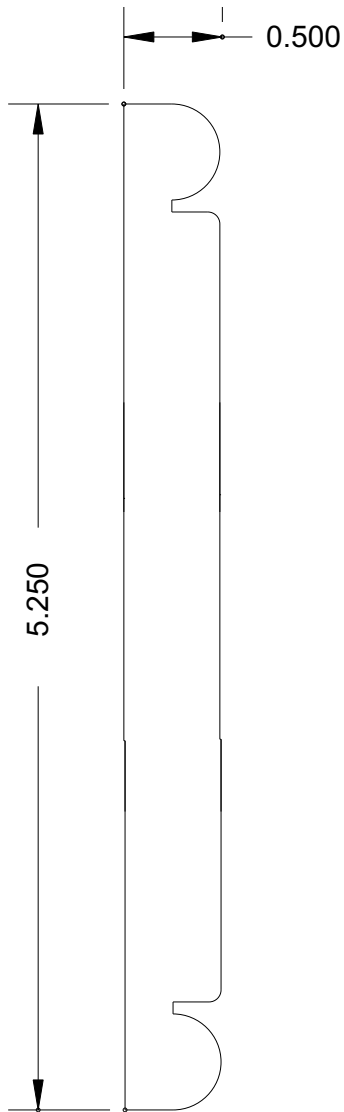
MB 969 (5-1/4 x 1/2)
