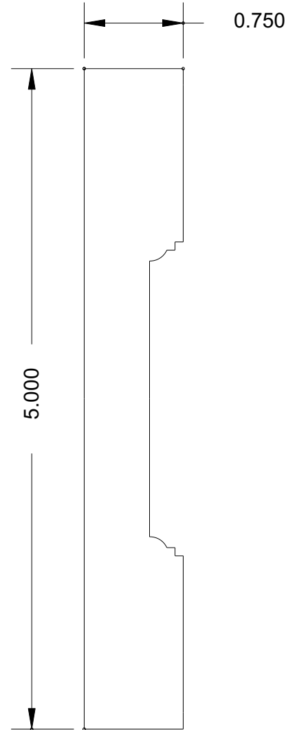
MB 979 (5 x 3/4)
