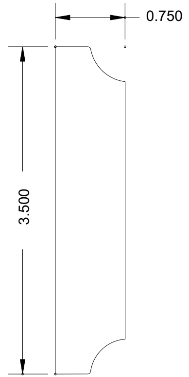
MB 6055 (3-1/2 x 3/4)
