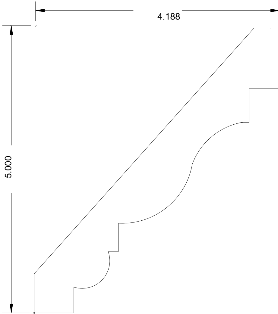
MB 1029 (6-1/2 x 15/16)
