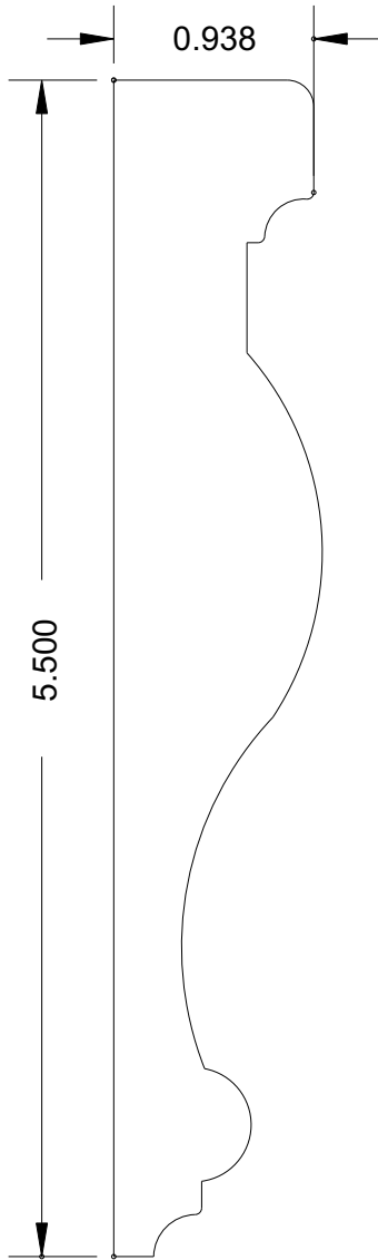
MB 6060 (5-1/2 x 15/16)
