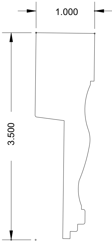
MB 6120 (3-1/2 x 1)
