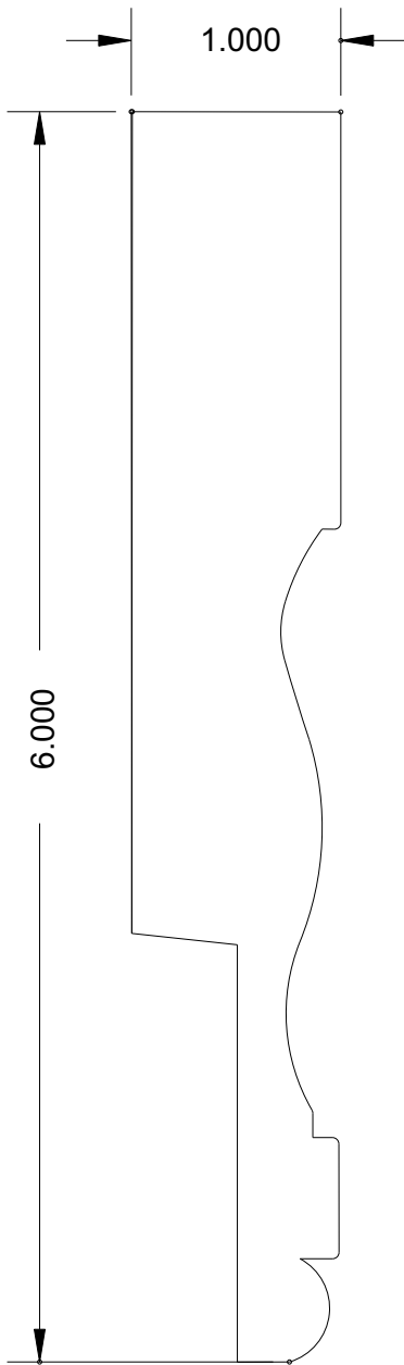
MB 647 (6 x 1)
