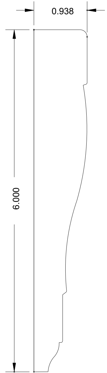
MB 678 (6 x 15/16)
