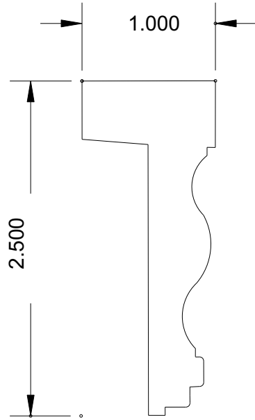
MB 6121 (2-1/2 x 1)
