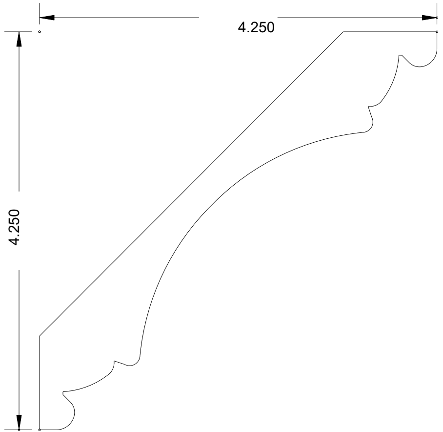
MB 1026 (6 x 15/16)
