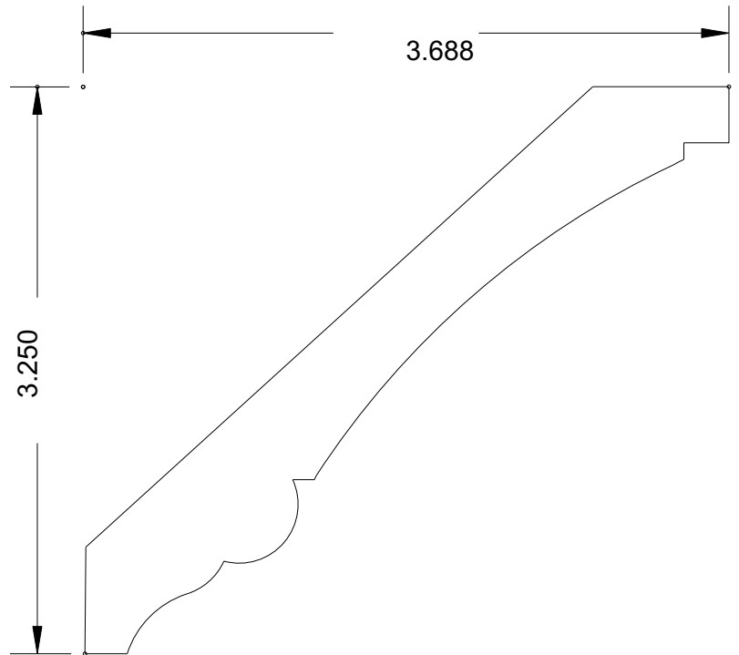
MB 1076 (4-7/8 x 11/16)
