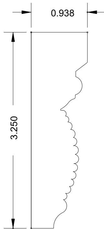
MB 651 (3-1/4 x 15/16)
