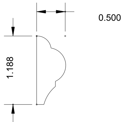
MB 4024 (1-3/16 x 1/2)
